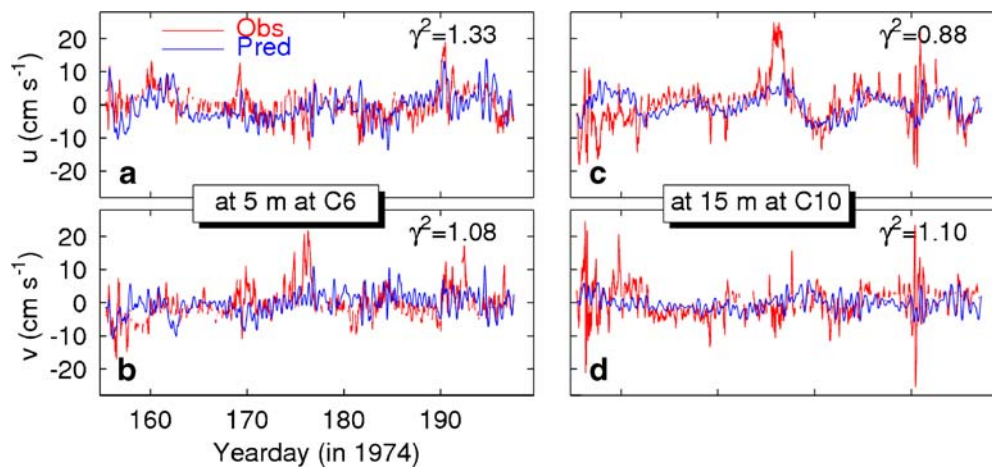
Fig. 15 Time series of model-predicted (blue plots) and observed (red plots) components of horizontal currents in depths of 5 m at site C6 (a and b) and 15 m at site C10 (c and d) in Bras d'Or Lake during the summer of 1974. The three-dimensional numerical model used for
