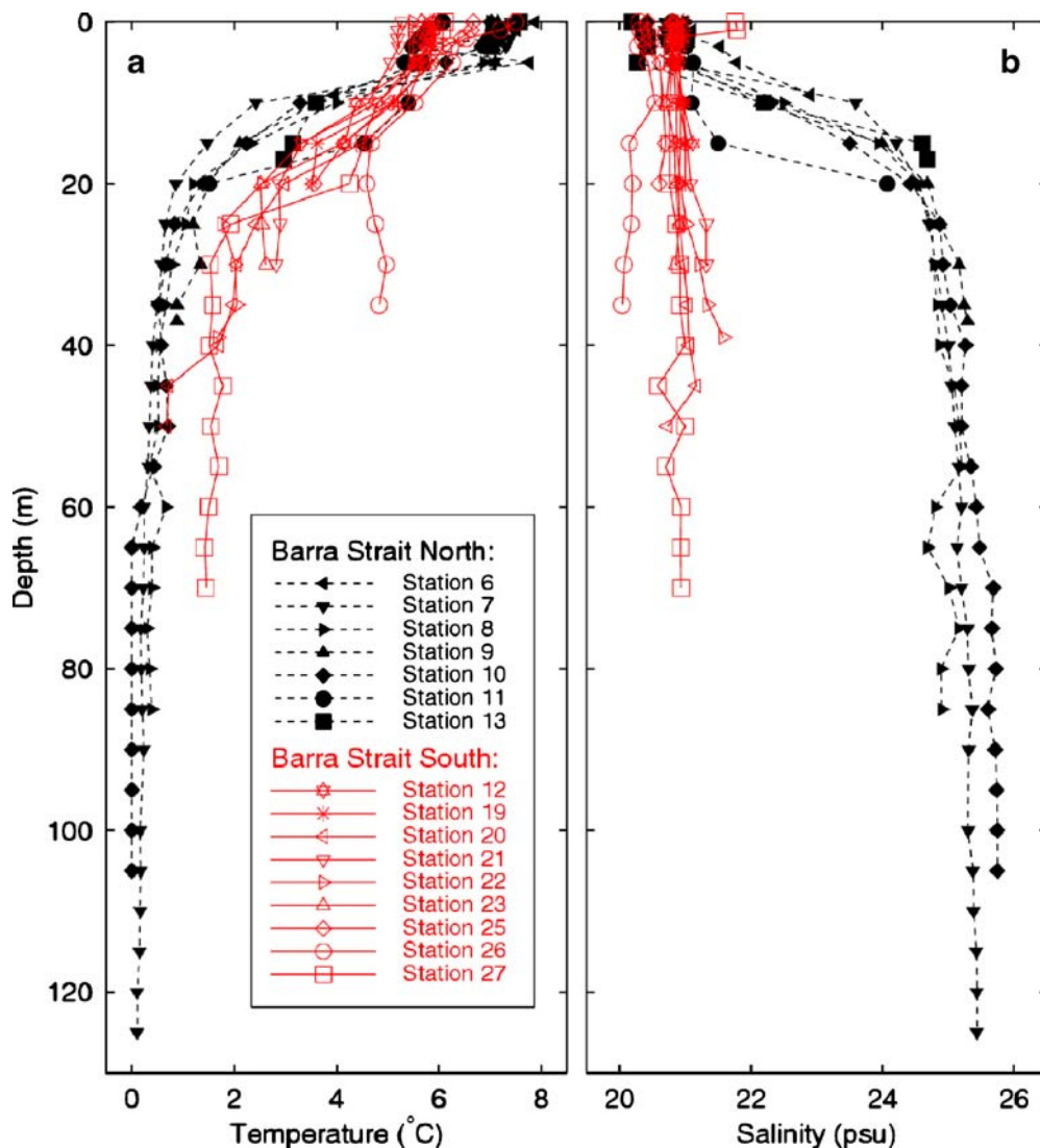
Fig. 3 Vertical profiles of a observed temperatures and b salinities in the Barra Strait separating the two great basins of the Bras d'Or estuary on May 22 and 23, 1974 (See Gurbutt and Petrie 1995 for the hydrographic locations)
