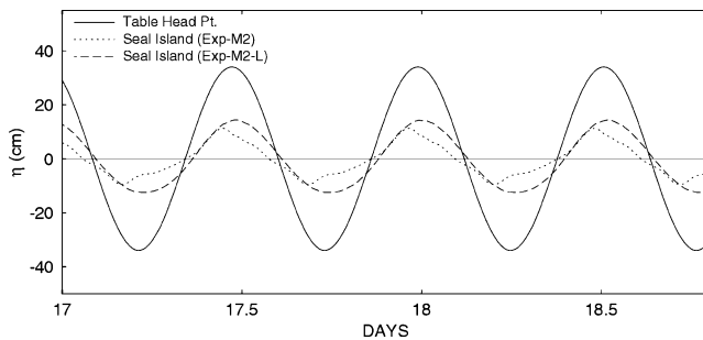
Fig. 8 Time series of surface elevations specified for Table Head Point at the northern open boundary ( solid line ) and model-calculated surface elevations at Seal Island in Exp-M2 ( dotted line ) and Exp-M2-L ( dashed line ). The time mean value is removed from each of the time series. The three-dimensional numerical circulation model used for the two experiments is forced by the M_2 tide at the model's northern open boundary
