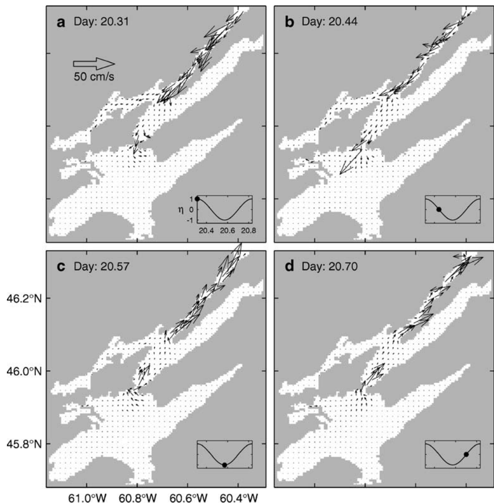
Fig. 4 Near-surface (2 m) currents at a day 20.31, b day 20.44, c day 20.57 and d day 20.70 in the Bras d'Or estuary (see Fig. 1) produced by the three-dimensional numerical circulation model in Exp-M2 (see Table 2). Current vectors are plotted at every third model grid. The model is forced by the M_2 tidal surface elevations specified at the northern open boundary. Insets show time series of sea levels at the northern open boundary, and the position in the tidal cycle is marked by the solid circle
