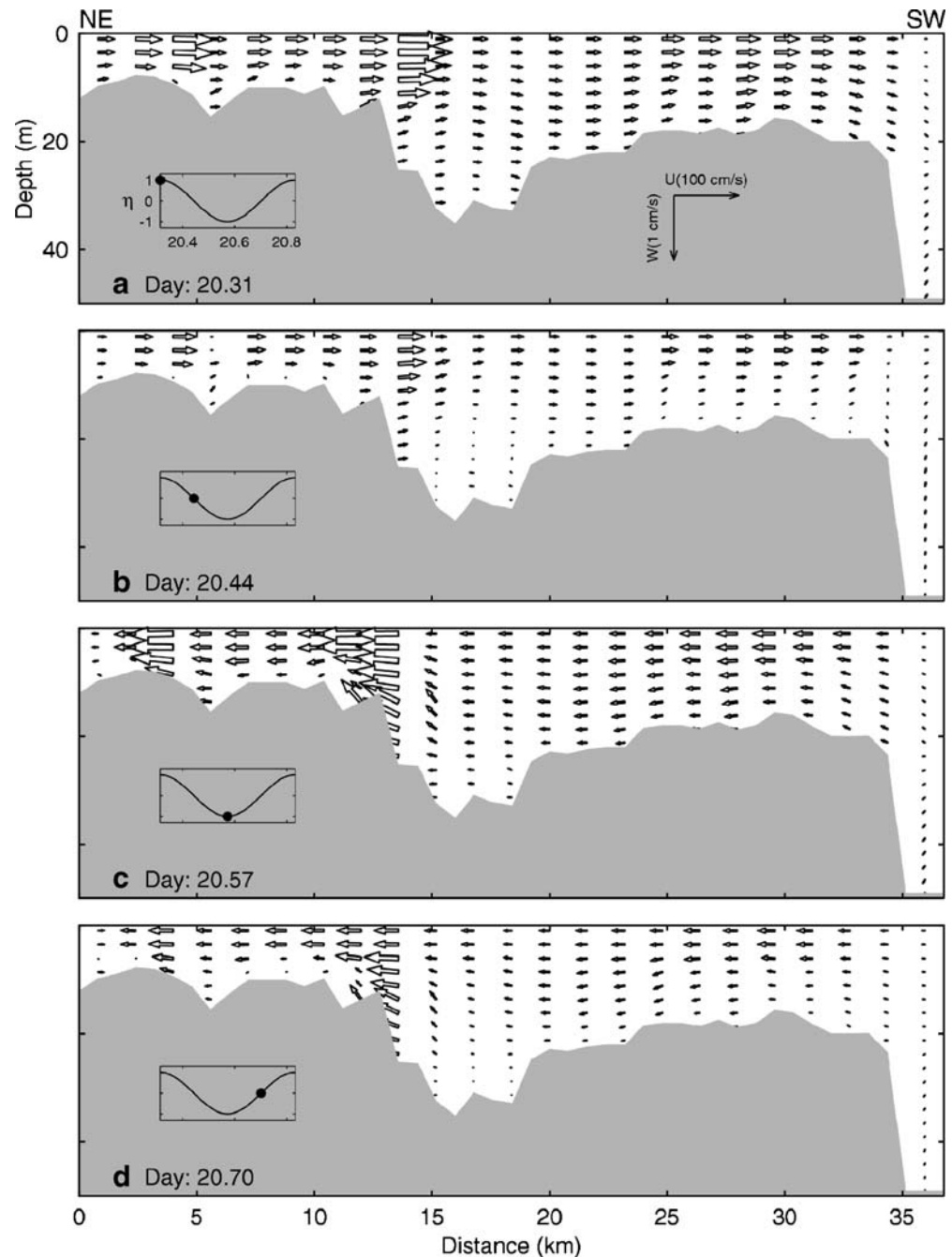
Fig. 5 Distributions of horizontal (along transect) and vertical components of tidal currents at a day 20.31, b day 20.44, c day 20.57 and d day 20.70 along the longitudinal axis of the Great Bras d'Or Channel (Fig. 1), produced by a three-dimensional numerical model in Exp-M2 (Table 2). The distance in the plots is measured from the NE end of transect. The model is forced by the M_2 tidal surface elevations specified at the northern open boundary. Insets show time series of sea levels at the northern open boundary, and the position in the tidal cycle is marked by the solid circle
