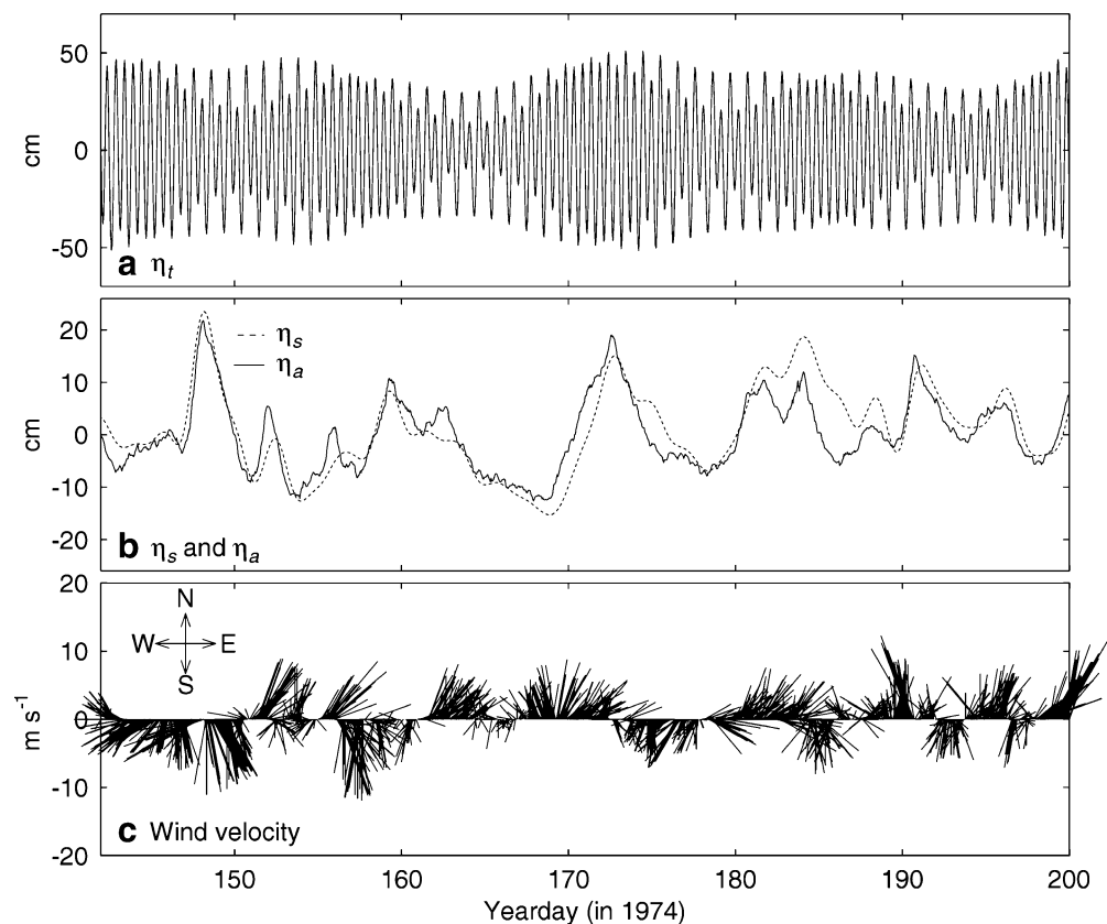
Fig. 2 Empirically measured forcing parameters used in driving a three-dimensional numerical circulation model of the Bras d'Or estuary. Time series of a tidal forcing \eta_t , b sub-tidal components of the observed sea levels ( \eta_s ) at North Sydney and sea level variations because of the inverse barometer effect ( \eta_a ) calculated from the air pressure measurements at Sydney Airport, and c observed wind velocity at Sydney Airport during the study period from 00:00 May 23 (day 142) to 00:00 July 20 (day 200) in 1974
