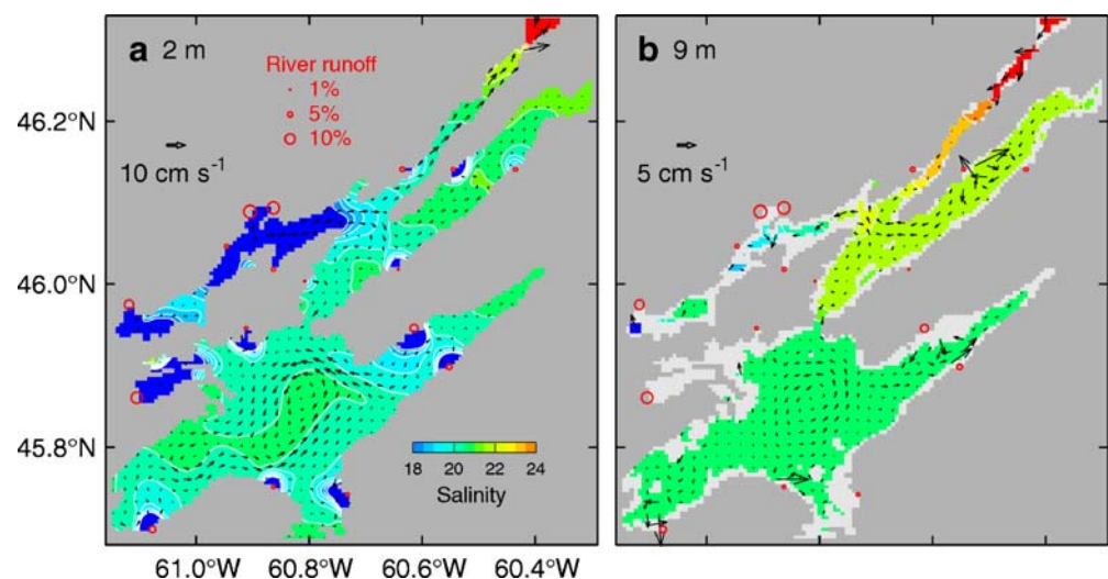
Fig. 12 Model-calculated a near-surface (2 m) currents and salinities and b sub-surface (9 m) currents and salinities at day 30 in a baroclinic run (Exp-R) of a three-dimensional numerical circulation model of the Bras d'Or estuary (Fig. 1) forced only by steady river runoff (Table 1). Velocity vectors are plotted at every third model grid
