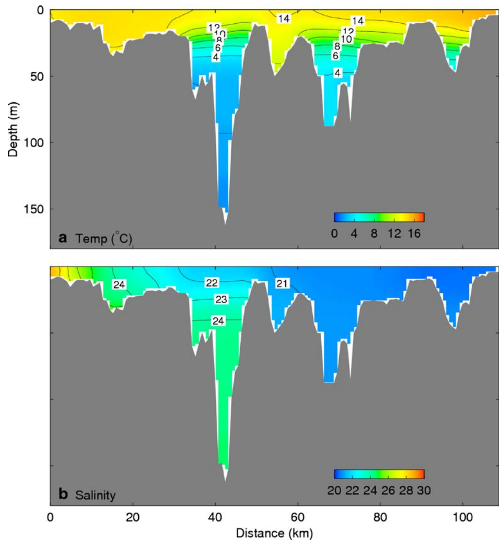
Fig. 17 Model-calculated (Exp-C) time-mean distributions of a temperature and b salinity along a transect from Table Head Point ( left ) to the head of East Bay ( right ) predicted for 15–19 July, 1974. The bathymetry of the Great Bras d’Or Channel, North Basin, Barra Strait, Bras d’Or Lake and East Bay are located from left to right . The distance in the plots is measured from the north end of transect. The white areas reflect the coarseness of the model grid scale relative to the resolution of the bathymetry. The three-dimensional numerical model used to generate this plot in Exp-C (Table 2) was driven by all-known forcing (i.e., tides, wind, buoyancy forcing and boundary flows associated with atmospheric pressure perturbations)
