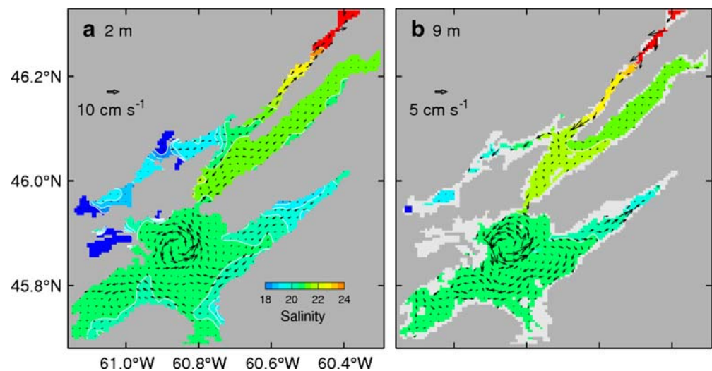
Fig. 19 Model-calculated density-driven currents and salinities in the a near-surface (2 m) layer and b sub-surface (9 m) layer in the Bras d'Or estuary during July, 1974. Velocity vectors are plotted at every third model grid. The three-dimensional numerical model used to generate this plot from Exp-D (Table 2) was initialized using temperature-salinity fields produced in Exp-C for 19 July, 1974 and ran for 3 days from rest with no external forcing
