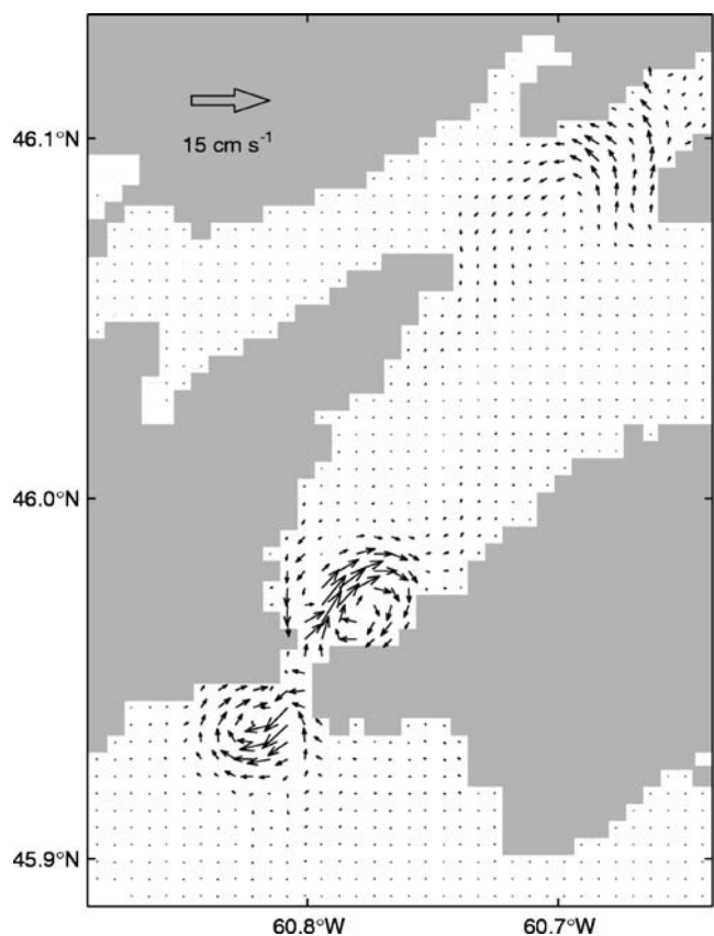
Fig. 9 Near-surface tidal residual flow in the vicinity of the Barra Strait (Fig. 1), as calculated from the model results of Exp-M2 (Table 2). The three-dimensional numerical model is forced by the M_2 tidal elevation specified at the model's open boundary. Current vectors are plotted at every model grid
