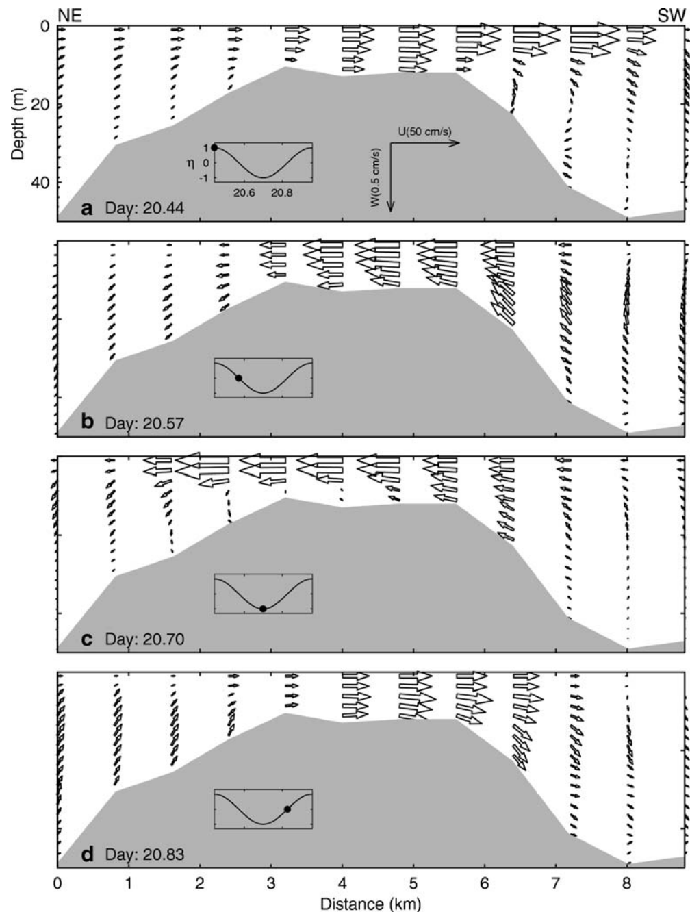
Fig. 6 Distributions of horizontal (along transect) and vertical components of tidal currents at a day 20.44, b day 20.57, c day 20.70 and d day 20.83 along the longitudinal axis of the Barra Strait (Fig. 1), produced by the three-dimensional numerical model in Exp-M2 (Table 2) at four phases of the M_2 tide. The distance in the plots is measured from the NE end of transect. The model is forced by the M_2 tidal surface elevations specified at the northern open boundary of the Great Bars d'Or Channel. Insets show time series of sea levels at the Iona, and the position in the tidal cycle is marked by the solid circle
