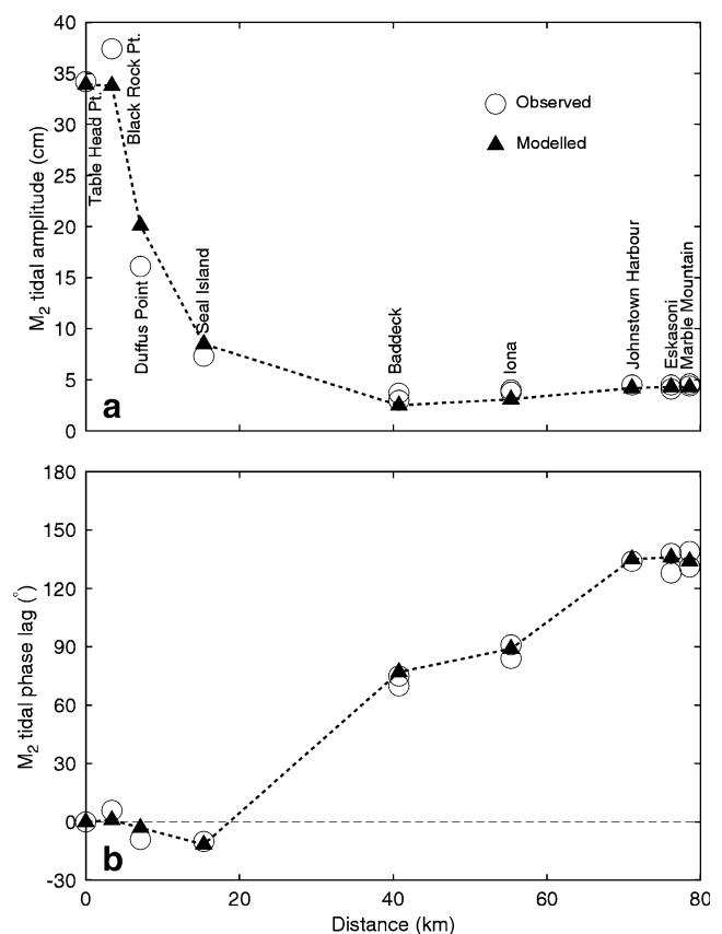
Fig. 7 Comparison of the observed ( open circles ) and model-calculated ( solid triangles ) a amplitudes and b phase lags relative to the tidal phase at Table Head Point of the M_2 surface elevations at nine locations along a transect from the mouth of the Great Bras d'Or Channel to the NE end of West Bay, Bras d'Or estuary (Fig. 1). The model is forced by the M_2 tidal surface elevations specified at the northern open boundary of the Great Bars d'Or Channel. The thin dashed line in b represents zero phase lag
