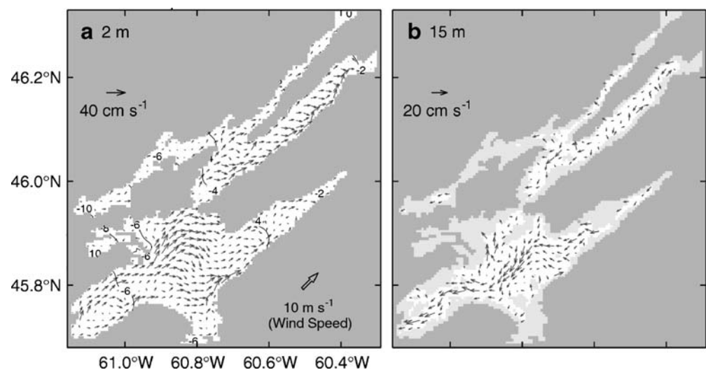
Fig. 11 Model-calculated a surface elevations and near-surface (2 m) currents and b sub-surface (15 m) currents at day 10 in a barotropic run (Exp-W) of a three-dimensional numerical circulation model of the Bras d'Or estuary (Fig. 1) forced only by steady northeastward winds of 10 \text{ m s}^{-1} . Contour interval for elevations is 2 cm. Velocity vectors are plotted at every third model grid
