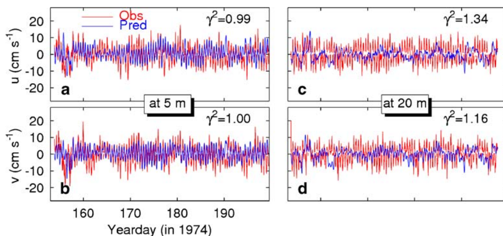
Fig. 14 Time series of model-predicted (blue plots) and observed (red plots) components of horizontal currents in depths of 5 (a and b) and 20 m (c and d) at site C3 in the North Basin of the Bras d'Or estuary during the summer of 1974. The three-dimensional numerical model
