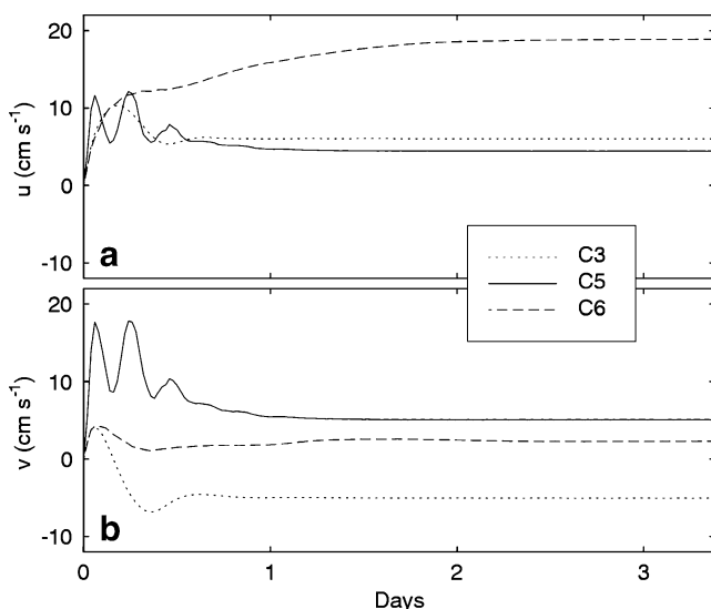
Fig. 10 Time series of a eastward and b northward components of the near-surface currents at locations C3, C5 and C6 along an oceanographic transect from the North Basin to Bras d'Or Lake (Fig. 1), produced by a circulation model in Exp-W (Table 2). The three-dimensional numerical model is forced only by the horizontally uniform and steady northeastward wind velocity of 10 \text{ m s}^{-1}
