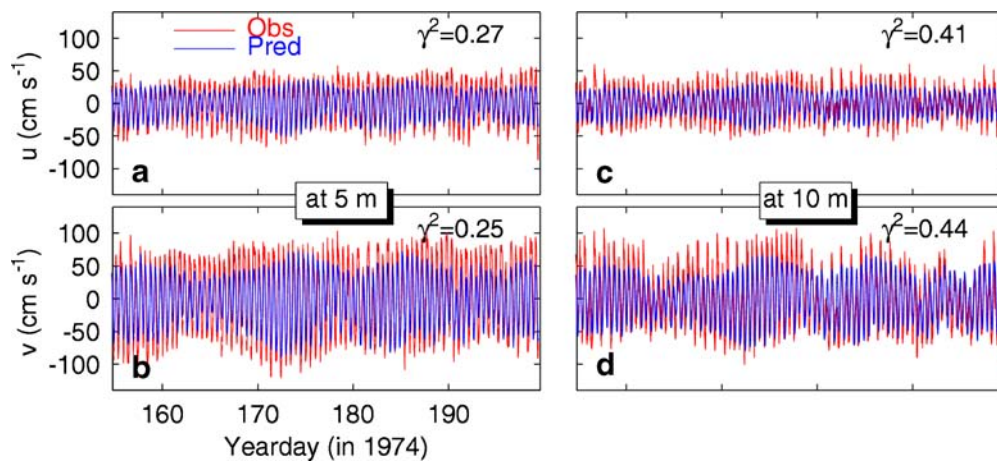
Fig. 13 Time series of scaled ( \times 1.3 ), model-predicted (blue plots) and observed (red plots) components of horizontal currents in depths of 5 (a and b) and 10 m (c and d) at site C5 in the Barra Strait during the summer of 1974. The three-dimensional numerical model used for
