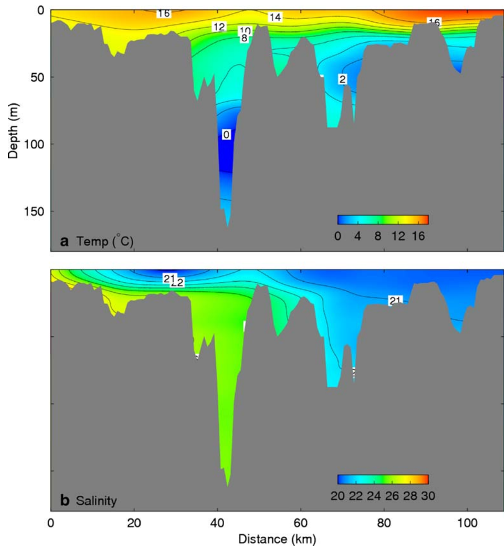
Fig. 16 Observed distributions of a temperature and b salinity along a transect from Table Head Point ( left ) to the head of East Bay ( right ) (see Fig. 1) during 15–19 July, 1974 made by Gurbutt and Petrie (1995). The bathymetry of the Great Bras d’Or Channel, North Basin, Barra Strait, Bras d’Or Lake and East Bay are located from left to right . The distance in the plots is measured from the north end of transect
